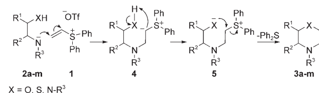
Scheme 1. Proposed annulation reaction for heterocycle synthesis mediated by vinyl sulfonium salt 1 .
